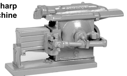
1968 Cincinnati 24" Shaper
